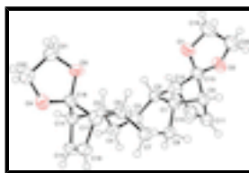
Fig. 2. A view of the molecular structure of compound 3 , with 50% probability displacement ellipsoids.
